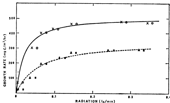
FIG. 5. Photosynthesis rate as a function of light intensity. From McAllister et al. (1964). The solid line is a best least-squares fit of equation (6) to the adjusted oxygen measurement, and the dashed line is a similar fit to carbon-14 measurements. The O and X represent the original and adjusted oxygen data, and the square and triangle represent respectively the original and adjusted carbon-14 data.
