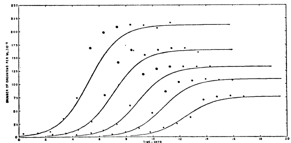
FIG. 4. Growth data for batch cultures of Isochrysis galbana with the initial nitrate specified in Table 1. The growth curves were fitted using equations (12).
