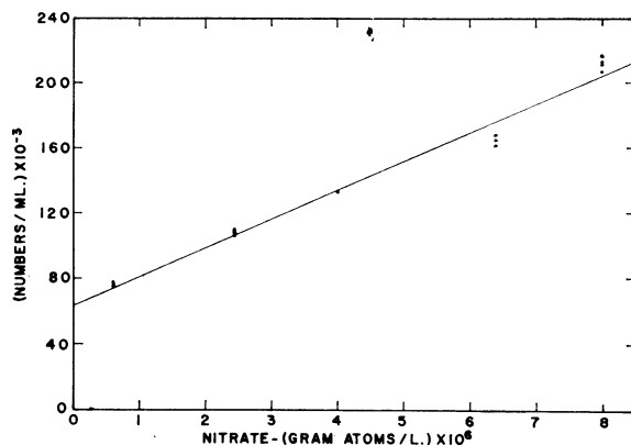
FIG. 2. Terminal population densities for the initial nitrate concentrations specified in Table 1. The slope of the best fit straight line provides an estimate of the yield coefficient, q .
