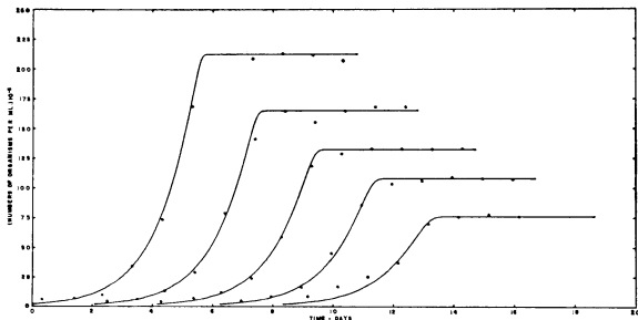
FIG. 3. Growth data for batch cultures of Isochrysis galbana with the initial nitrate concentration specified in Table 1. The growth curves were fitted using equations (10) and (11).
