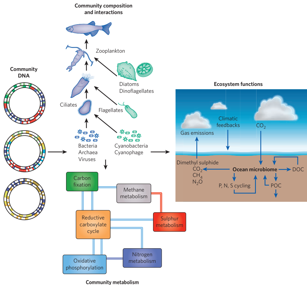
Figure 4 | The network instructions encoded in microbial genomes drive ecosystem processes. This schema shows hypothetical linkages between the genomic information of the microbial assemblage and the collective ecological interactions and community metabolism that in part regulate and sustain biogeochemical and ecosystem processes. Each DNA circle in
